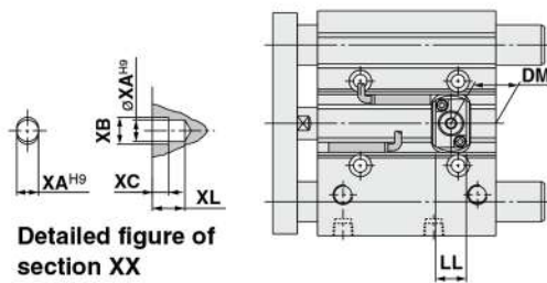
With head end lock
