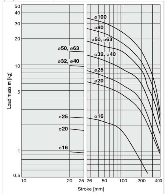
(16) L = 100 mm, V = 200 mm/s or less
