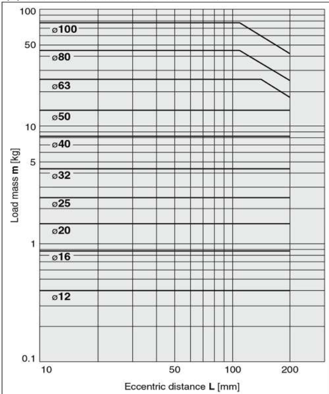
(3) 50 stroke or less, V = 400 mm/s
