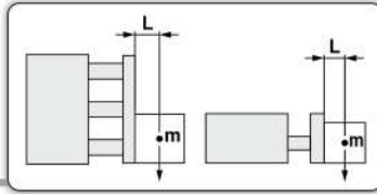
(14) L = 100 mm, V = 200 mm/s or less
