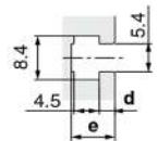
T-slot dimensions [mm]
