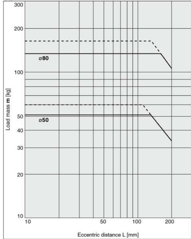
(2) Over 50 Stroke, V = 200 mm/s or less
