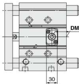
With head end lock
