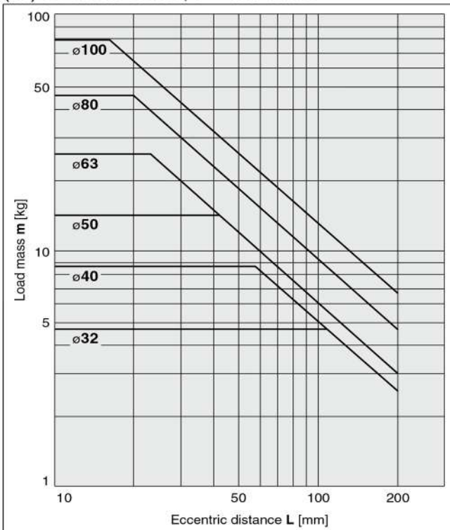
(11) 50 stroke or less, V = 400 mm/s
