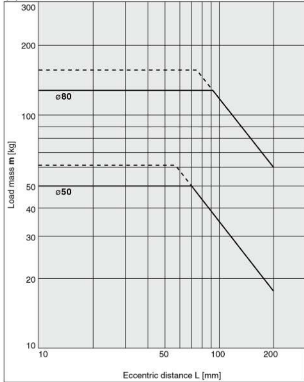
(1) 50 Stroke or Less, V = 200 mm/s or less
