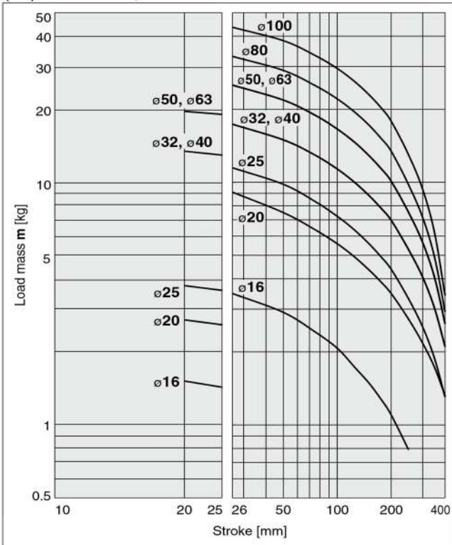
(15) L = 50 mm, V = 200 mm/s or less
